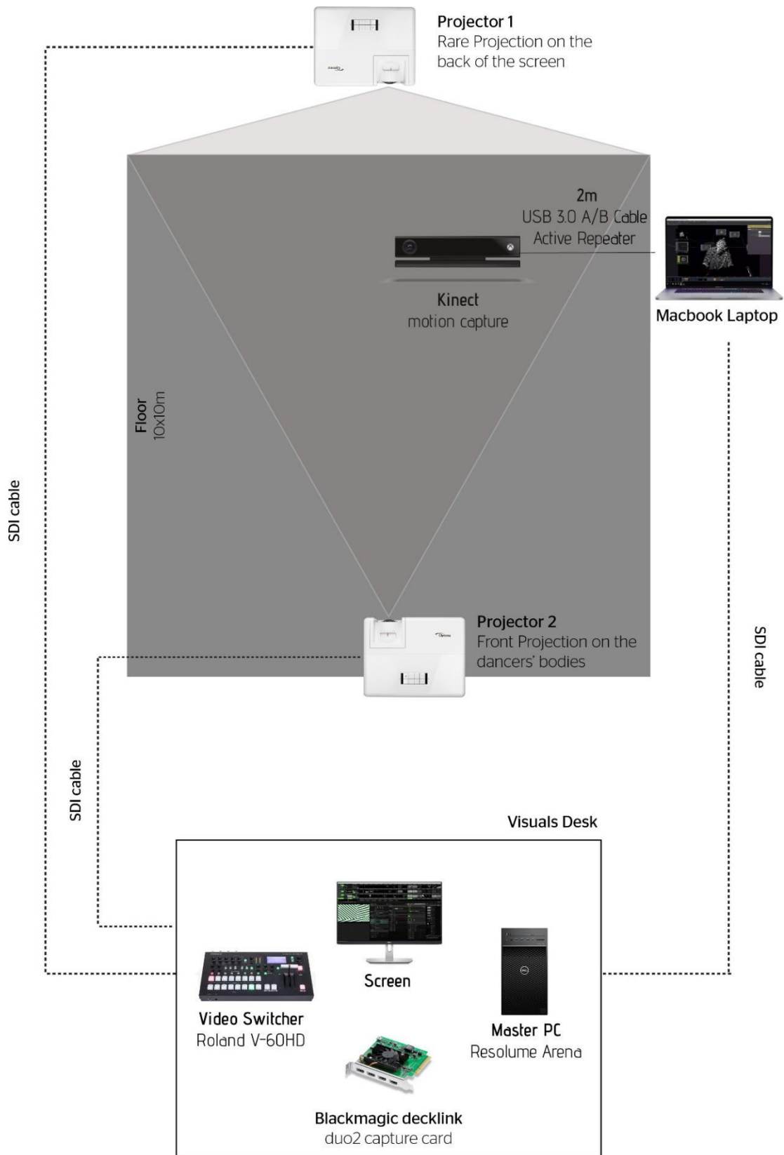
Figure 1: setup diagram
